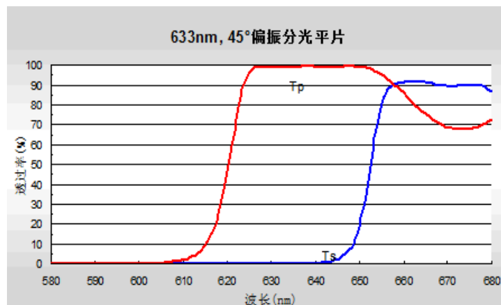
透射谱(633nm)
