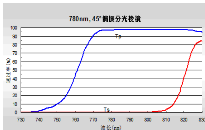
透射谱(780nm)
